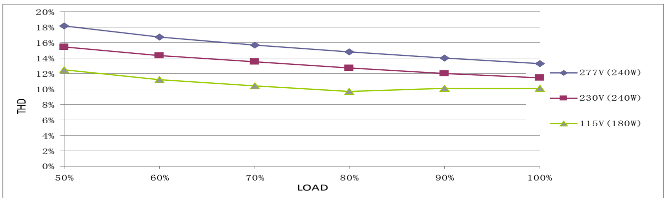
THD vs LOAD
