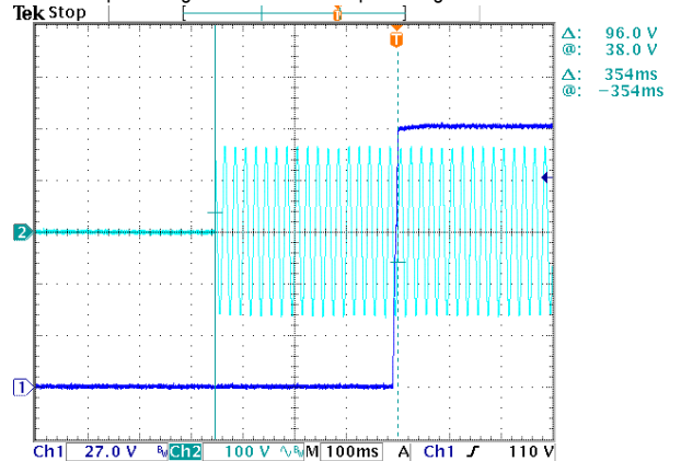
INPUT=115VAC/60HZ @ 75% LOAD
